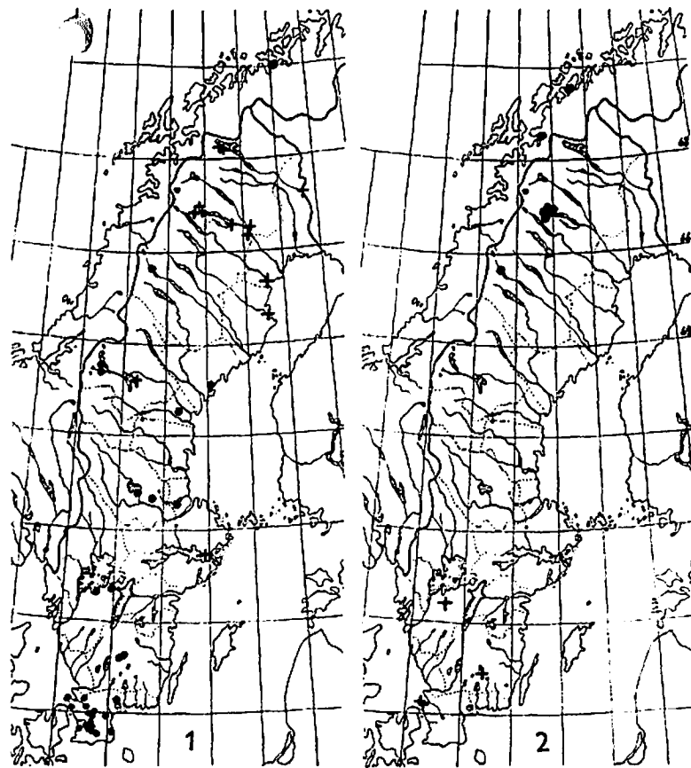
Fig. 1—2. Distribution in Sweden and northernmost Norway of 1) Beris strobli Dušek & (+) and Beris chalybeata Forst. (•); 2) Beris morrisi Dale (+) and Beris fuscipes Meig
